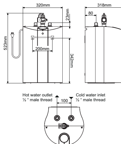
SHC 15 AU under sink compact storage water heater
