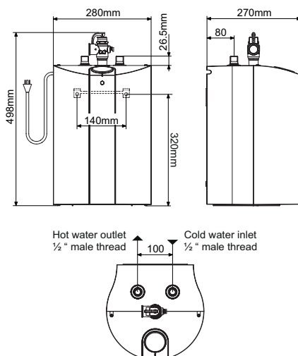
SHC 10 AU under sink compact storage water heater
