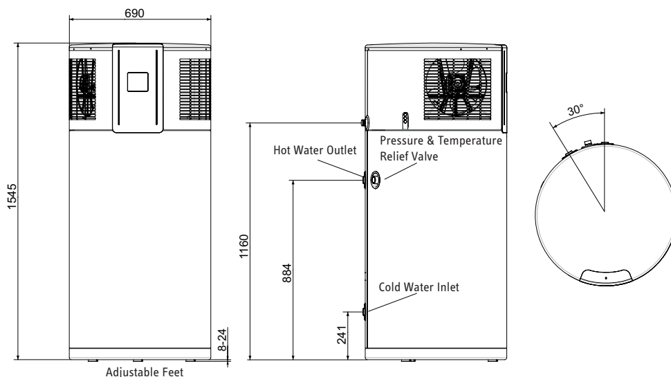
WWK 222 | WWK 222H hot water heat pump
